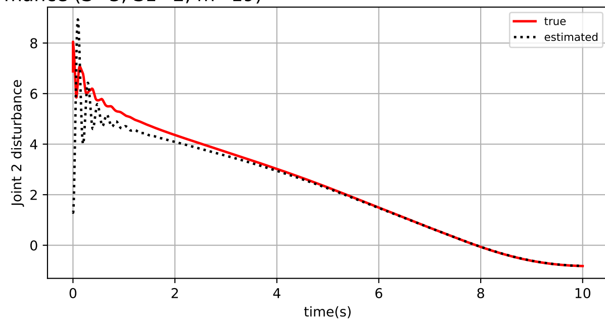
Disturbance Estimation Performance (S=3, S1=2, m=19)
