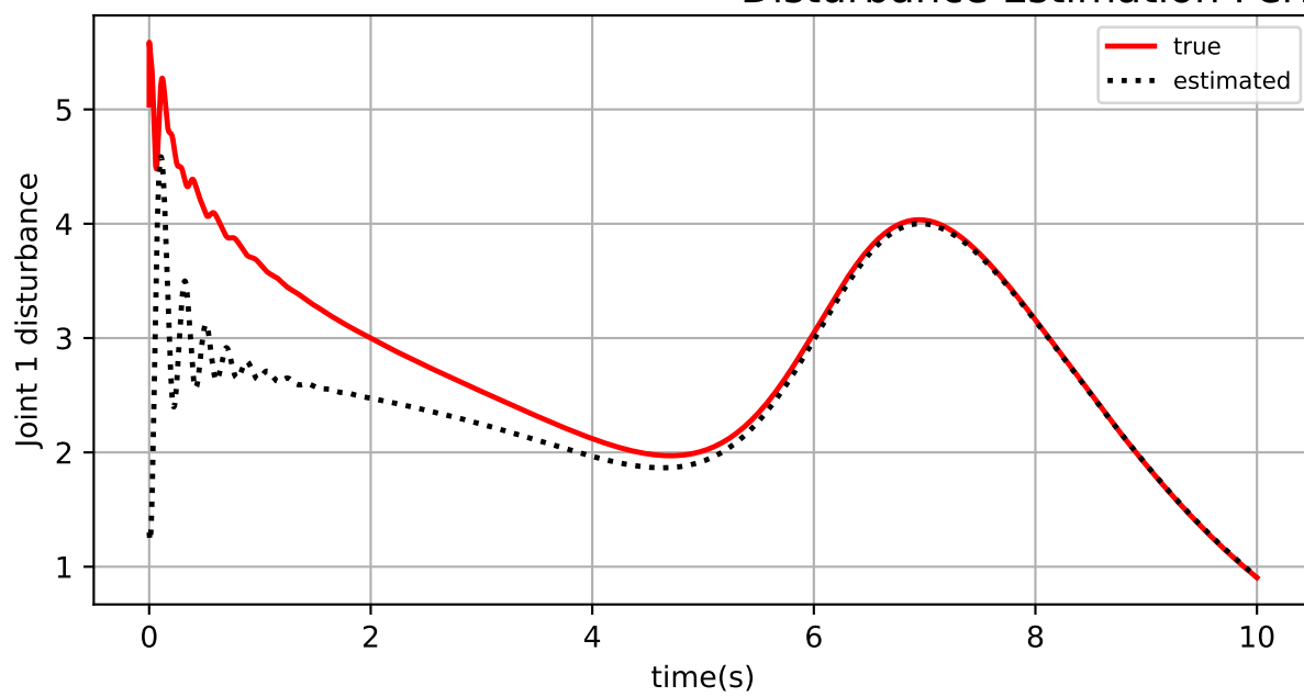
Disturbance Estimation Performance (S=3, S1=2, m=19)
